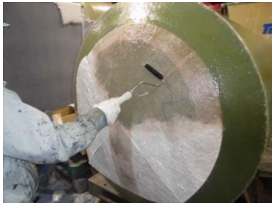
Hand Lay up method
